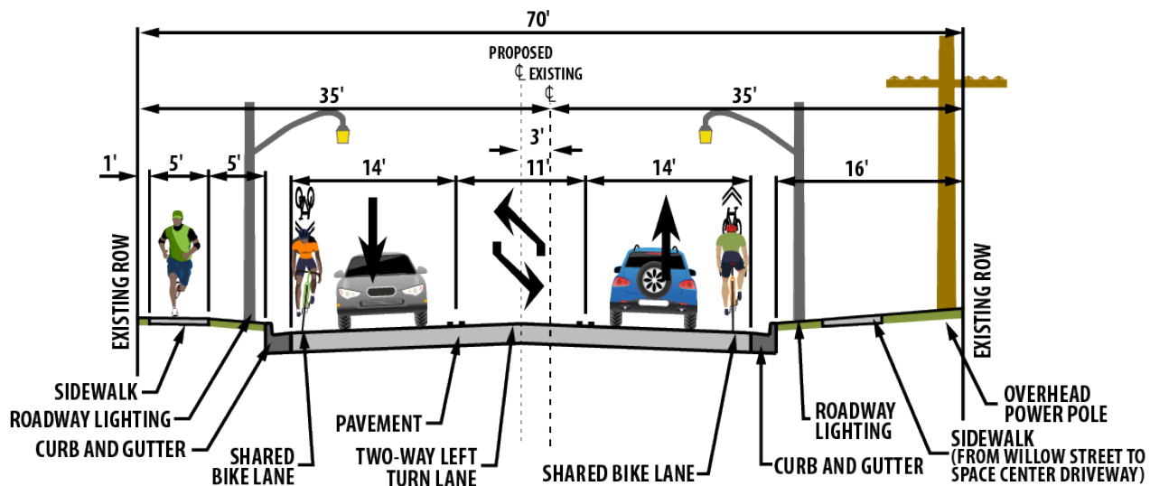
HOBBIE AVENUE PROPOSED TYPICAL SECTION (WILLOW STREET TO FAIR STREET)
