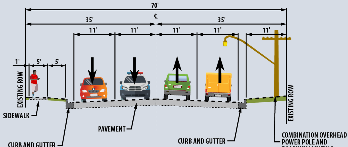
HOBBIE AVENUE EXISTING TYPICAL SECTION (WILLOW STREET TO FAIR STREET)
